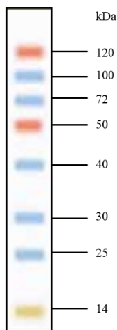
12% SDS-PAGE (5ul/well)
